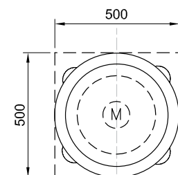
TurboSwing 750 / 1100
