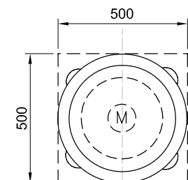
UV Turbo 750 / 1100
